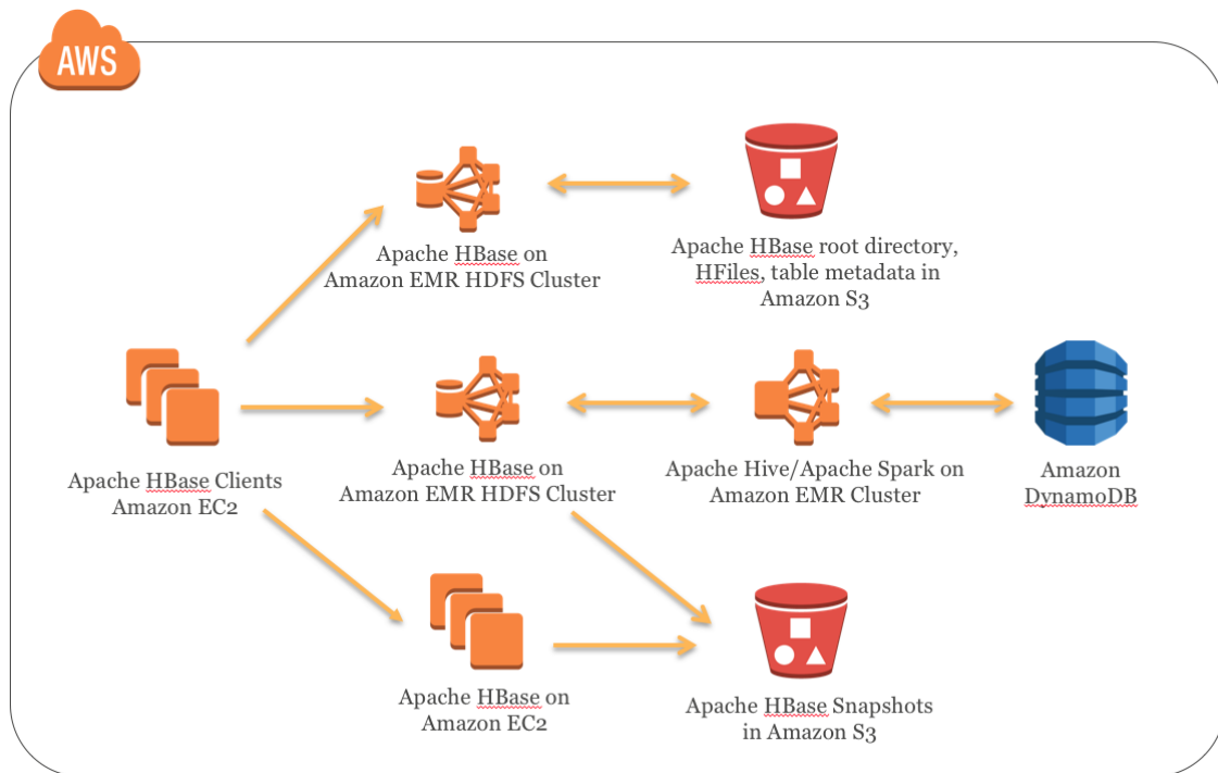
Figure 1: Relation of AWS, Amazon DynamoDB, Amazon EC2, Amazon EMR, and Apache HBase
