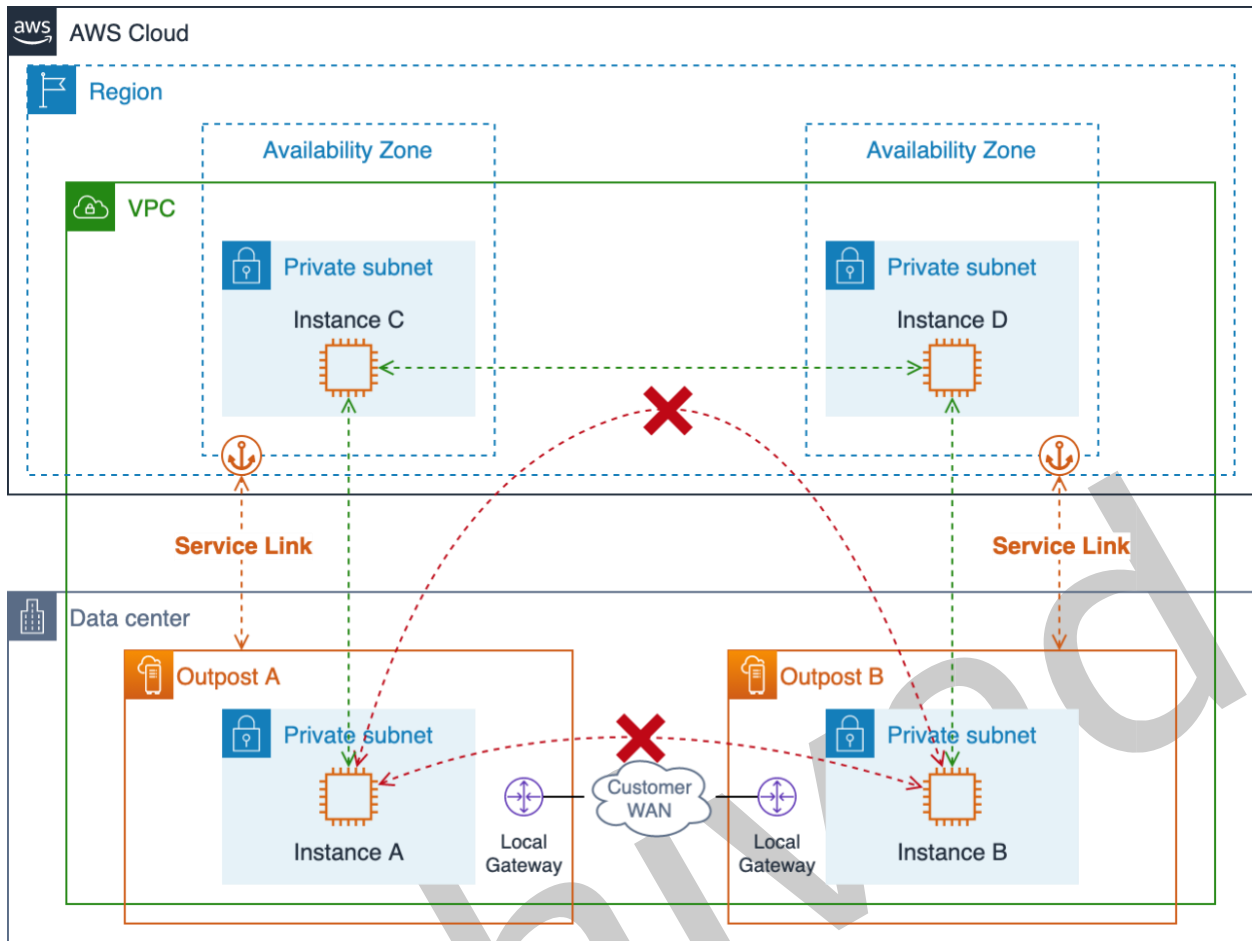
Single VPC multiple-outpost network paths
