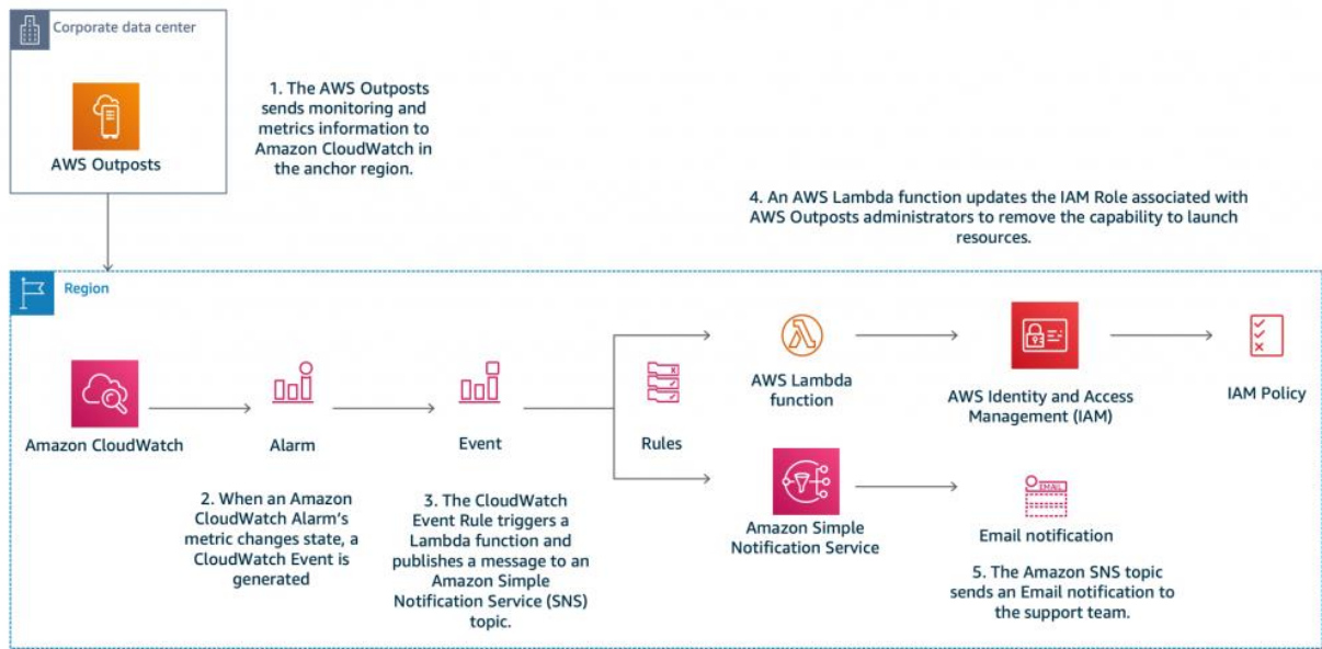
Managing AWS Outposts capacity with Amazon CloudWatch and AWS Lambda
