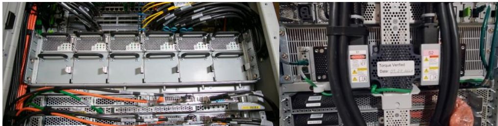
Figure 1 - AWS Outposts AC-to-DC power supplies and bus bar power distribution
