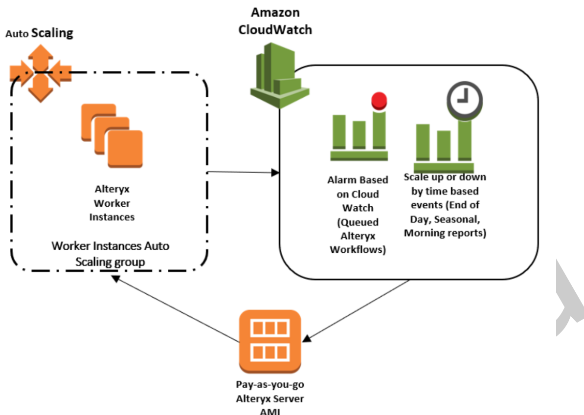
Figure 4: Use Amazon EC2 Auto Scaling and Amazon CloudWatch to scale Worker instances on-demand
