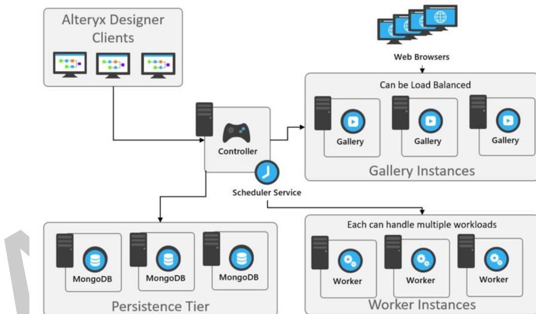
Figure 1: Scalable enterprise deployment of Alteryx Server
