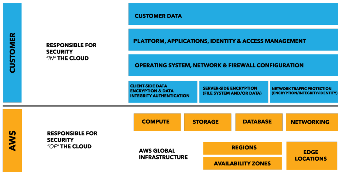
Figure 1: The AWS Shared Responsibility Model
