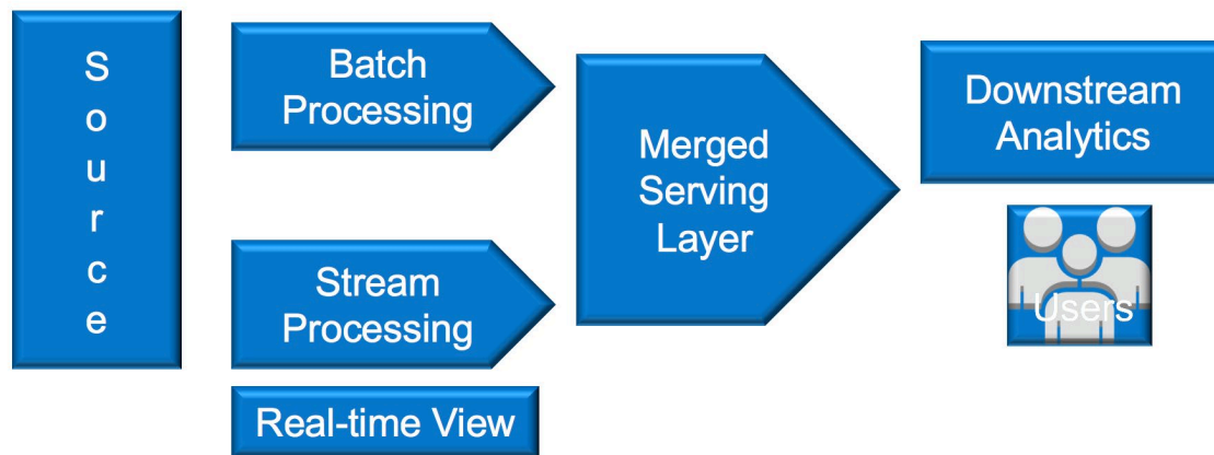
Figure 1: Lambda Architecture
